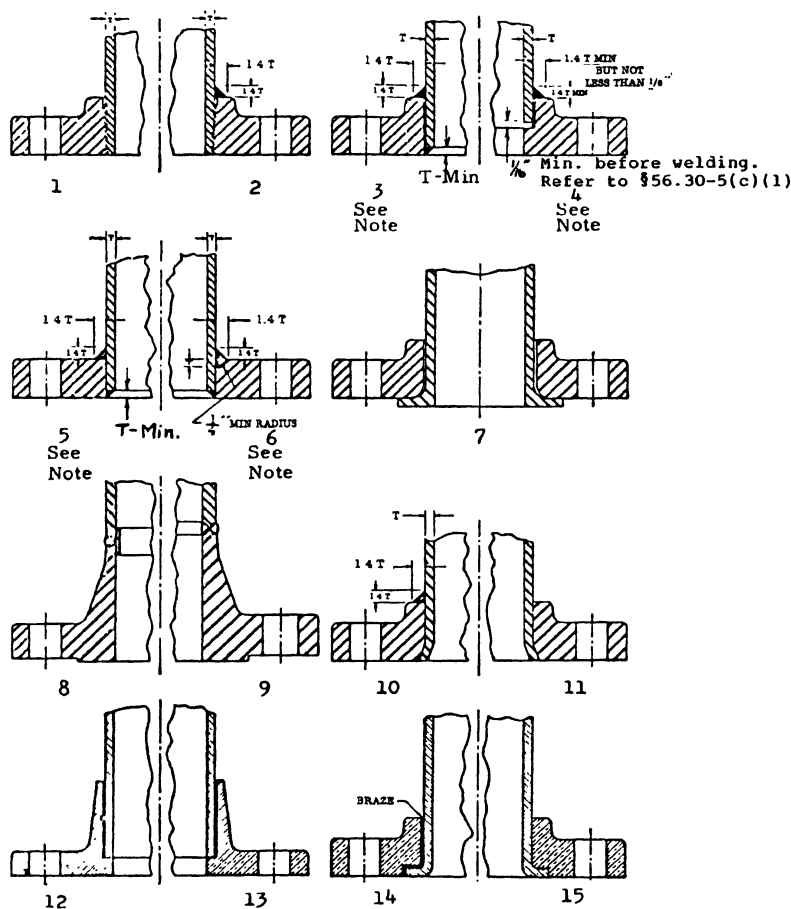
Figure 56.30-10(b)—Methods of Attachment
